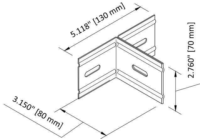
TUBRISE FOLDED BRACKET
